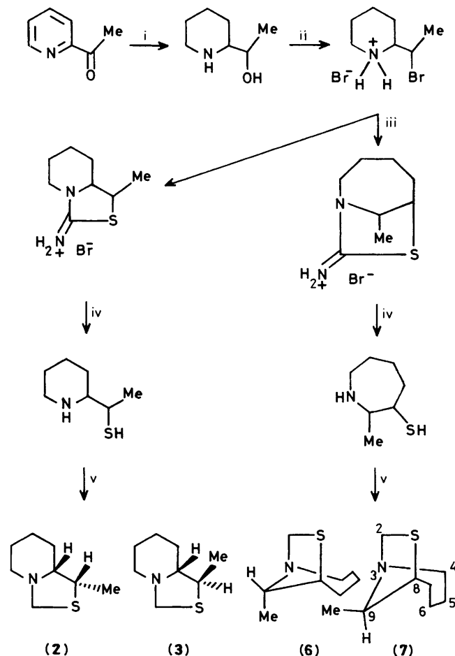
Scheme. Synthesis of the 1-methylperhydrothiazolo[3,4- a ]pyridines and 9-methylperhydro-3,8-methano-1,3-thiazocines. Reagents: i, H 2 -PtO 2 ; ii, HBr-PBr 3 ; iii, thiourea; iv, tetraethylenepentamine; v, aqueous CH 2 O
